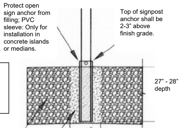
Galvanized Post Detail
